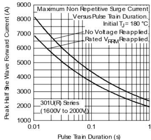
Fig. 10 - Maximum Non-Replicative Surge Current
