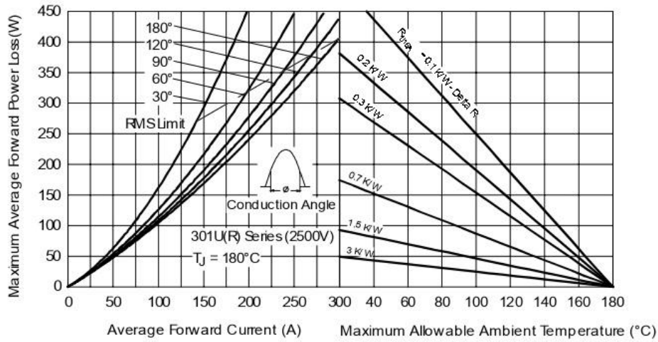
Fig. 7 - Forward Power Loss Characteristics
