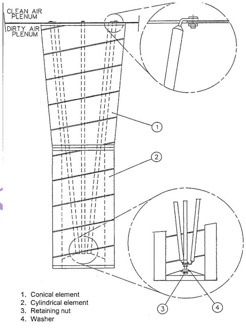
Fig: GT Intake Air Filter element and fixation picture.
