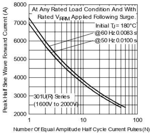
Fig. 9 - Maximum Non-Replicative Surge Current
