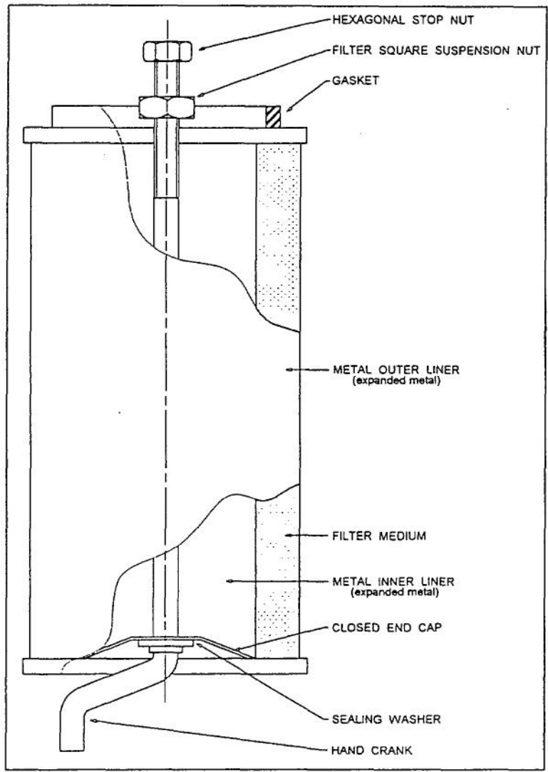
Fig: Generator Air Filter (Cylindrical) Drawing.
